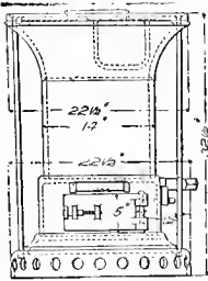
Fig. 3068a. Elevation.
